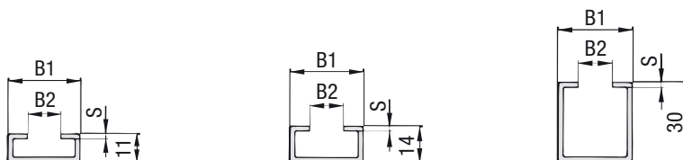
Mounting Rail TS 11
